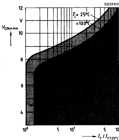
Figure 12. Typical static inhibit voltage limit V_{DINHmin}=f(I_F/I_{FT25^\circ C}) , parameter: T_j Device zero voltage switch can be triggered only in hatched area below T_j curves.
