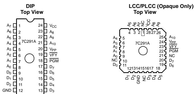
Figure 1. Programming Pinouts
