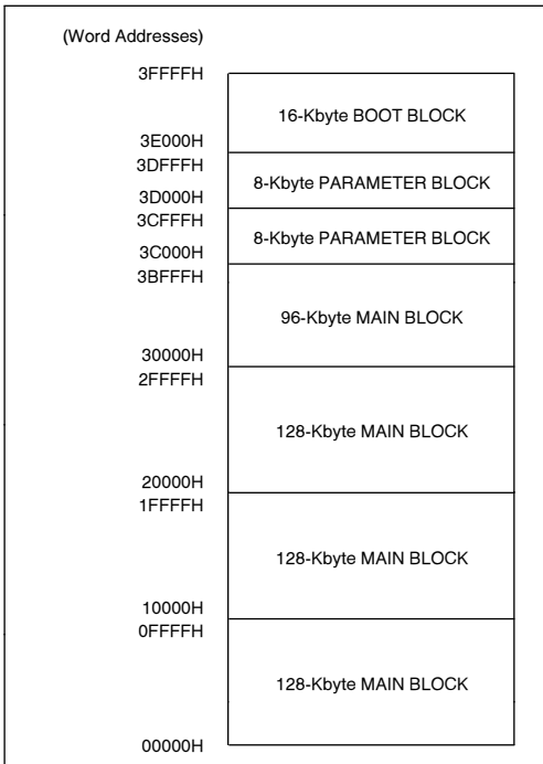
Figure 5. A28F400BX-T Memory Map
