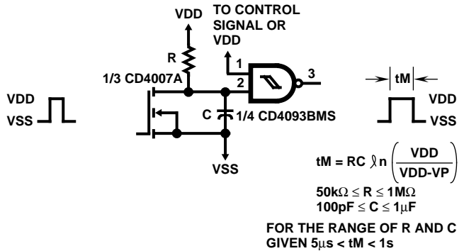
FIGURE 16. MONOSTABLE MULTIVIBRATOR
