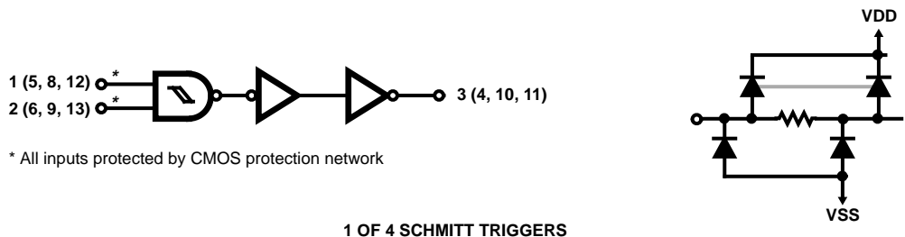
1 OF 4 SCHMITT TRIGGERS
