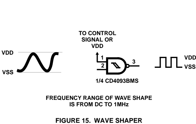
FIGURE 15. WAVE SHAPER
