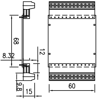
TERMINALS
