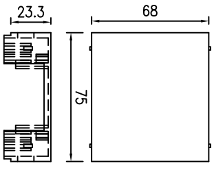
TOP COVER
