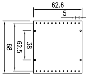
TERMINAL PCB
