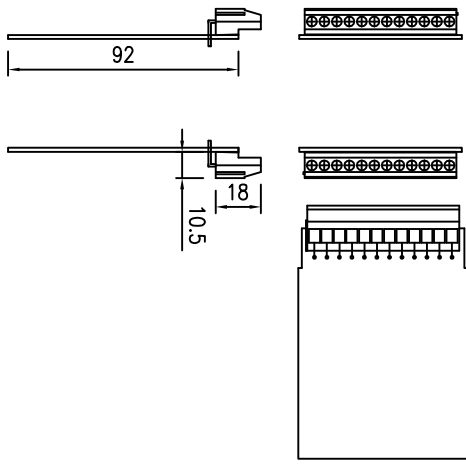
TERMINALS
