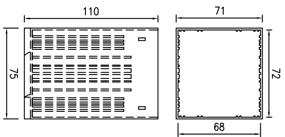
CASE BODY
