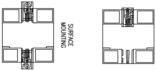
RAIL MOUNTING
