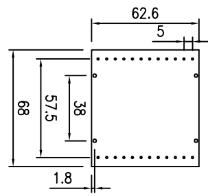
TERMINAL PCB
