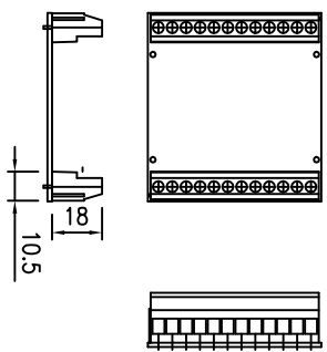
TERMINALS
